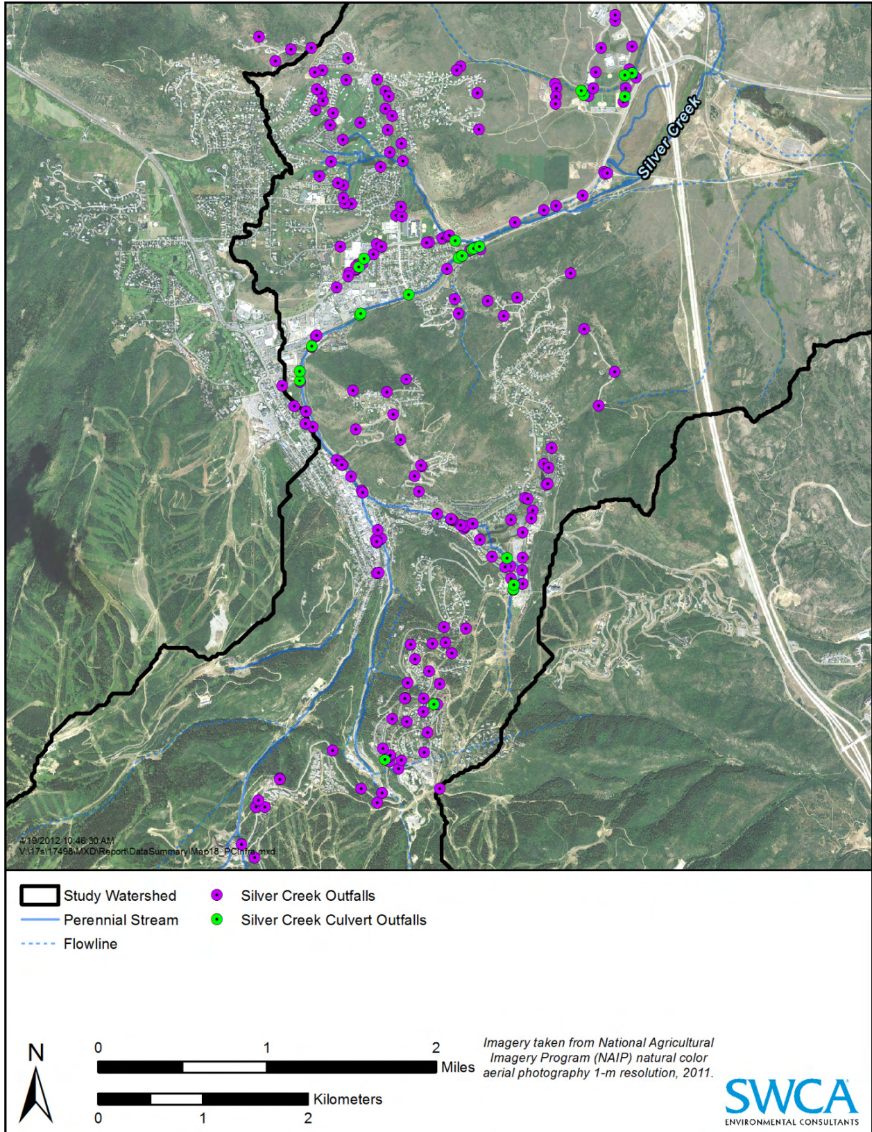
Figure 4. Locations of stormwater outfalls in the Silver Creek subwatershed.
