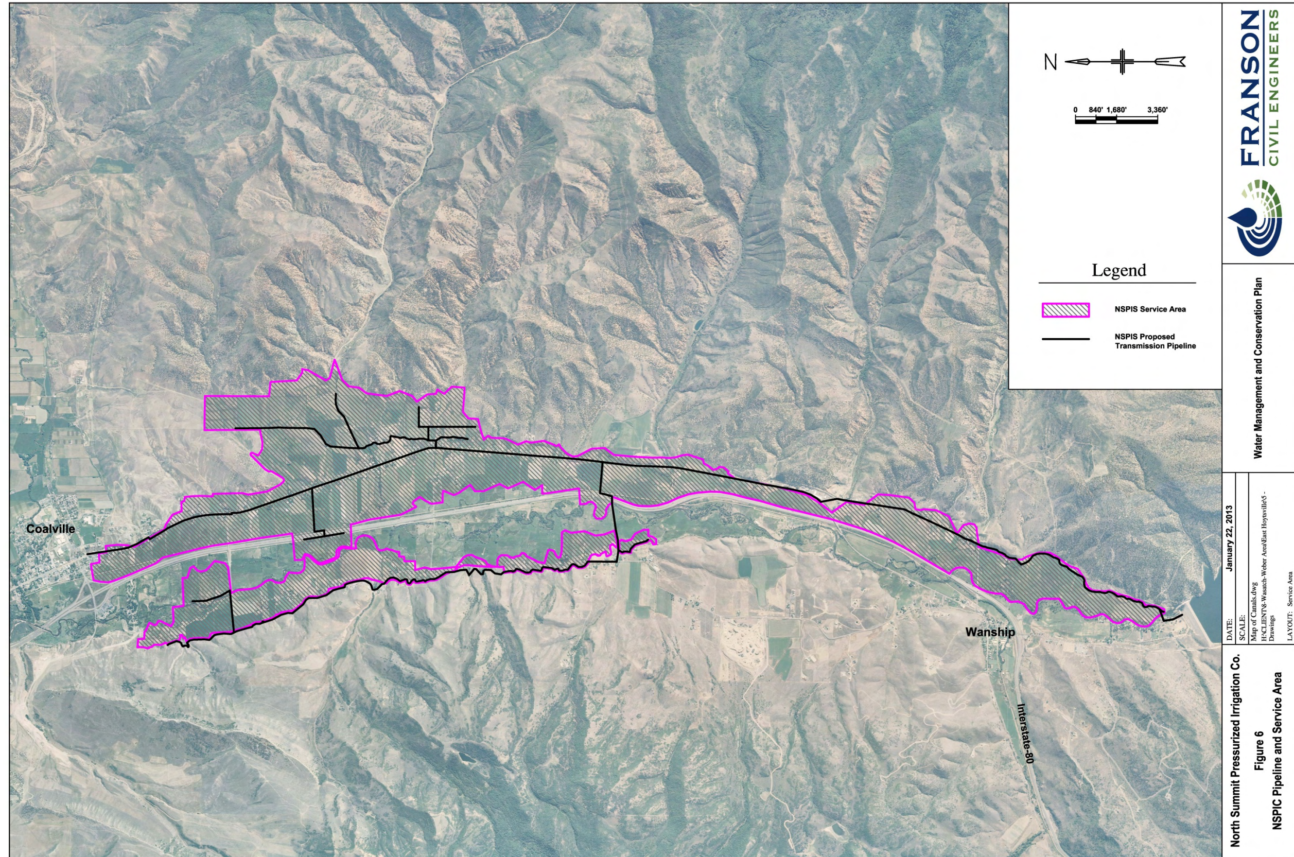
Figure 17. Proposed pipeline route and service area for North Summit Pressurized Irrigation System (Source: Layne Jensen, Franson Civil Engineering, 2013).
